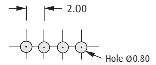
Recommended PC Board Pattern
