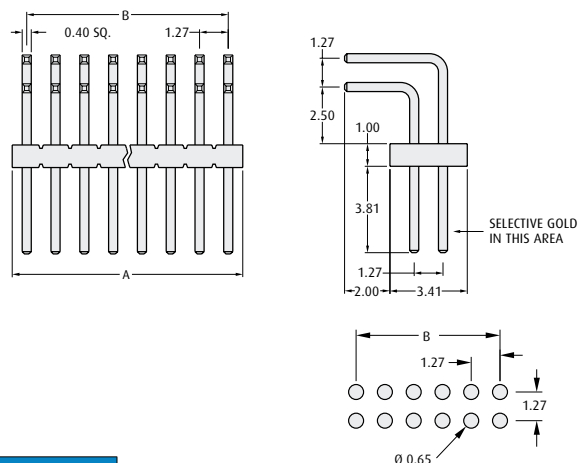
Recommended PC Board Pattern
