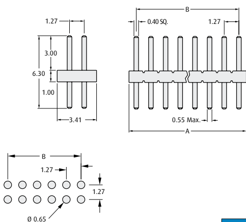
Recommended PC Board Pattern
