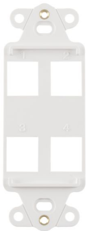
Rectangular Decorator 4 Port Mounting Frame, ABS 94V-0, White, 1/pkg
