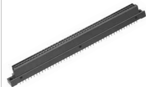
PCN10MC-*S-2.54DSA(72)
