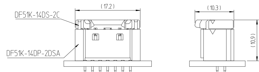
ENGAGEMENT FIGURE (2:1)
