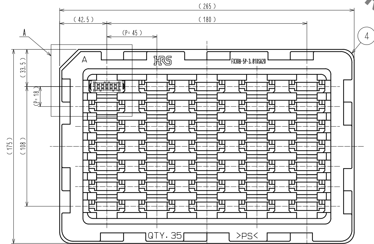
1 Drawing for packaging(1:2)
