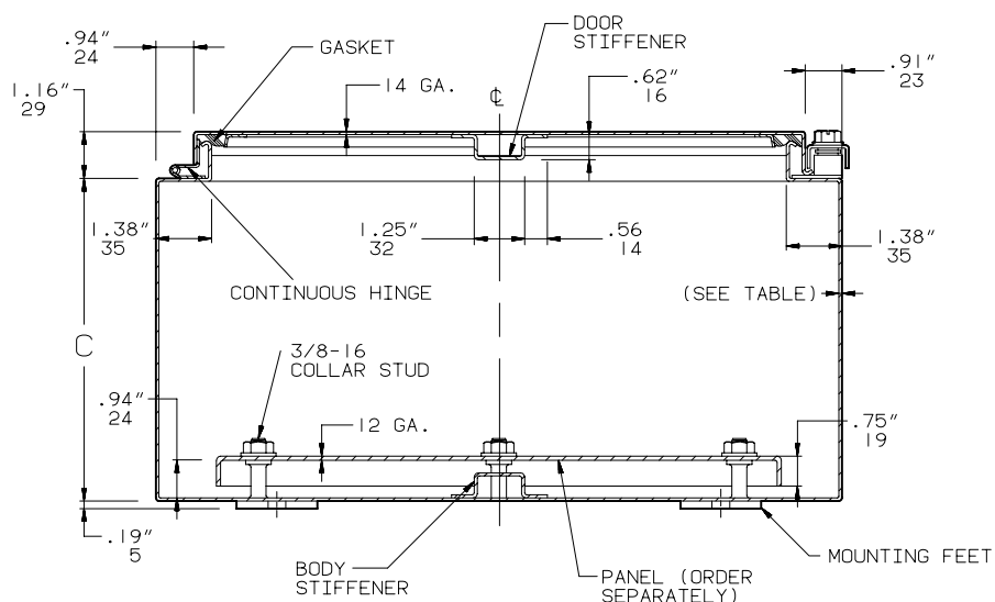
SECTION X-X
