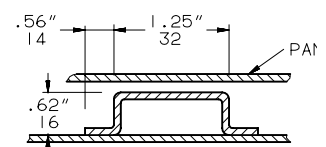
SECTION Z-Z
