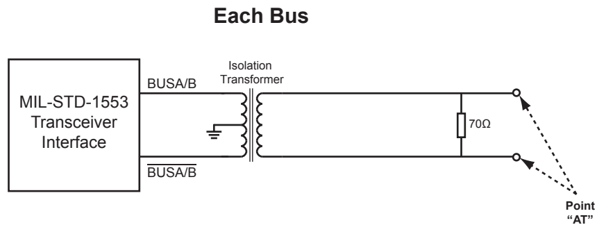
Figure 8. MIL-STD-1553 Transformer Coupled Test Circuit Example
