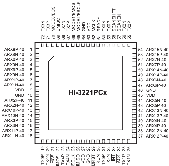
72 - Pin Plastic QFN (Top View)
