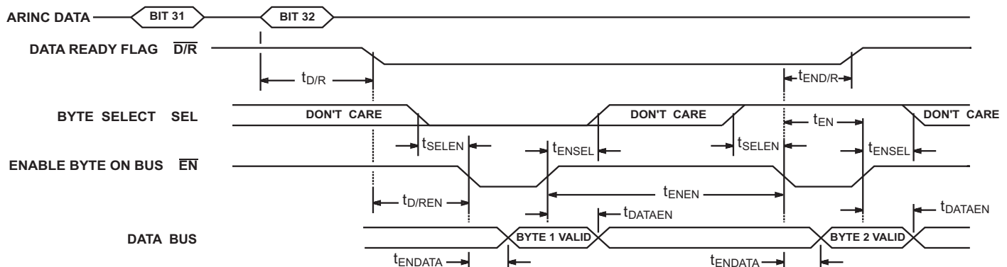
RECEIVER OPERATION
