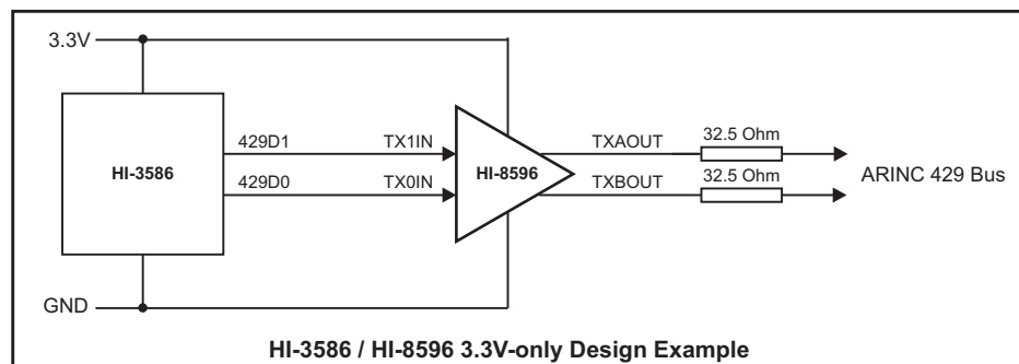
HI-3586 / HI-8596 3.3V-only Design Example
