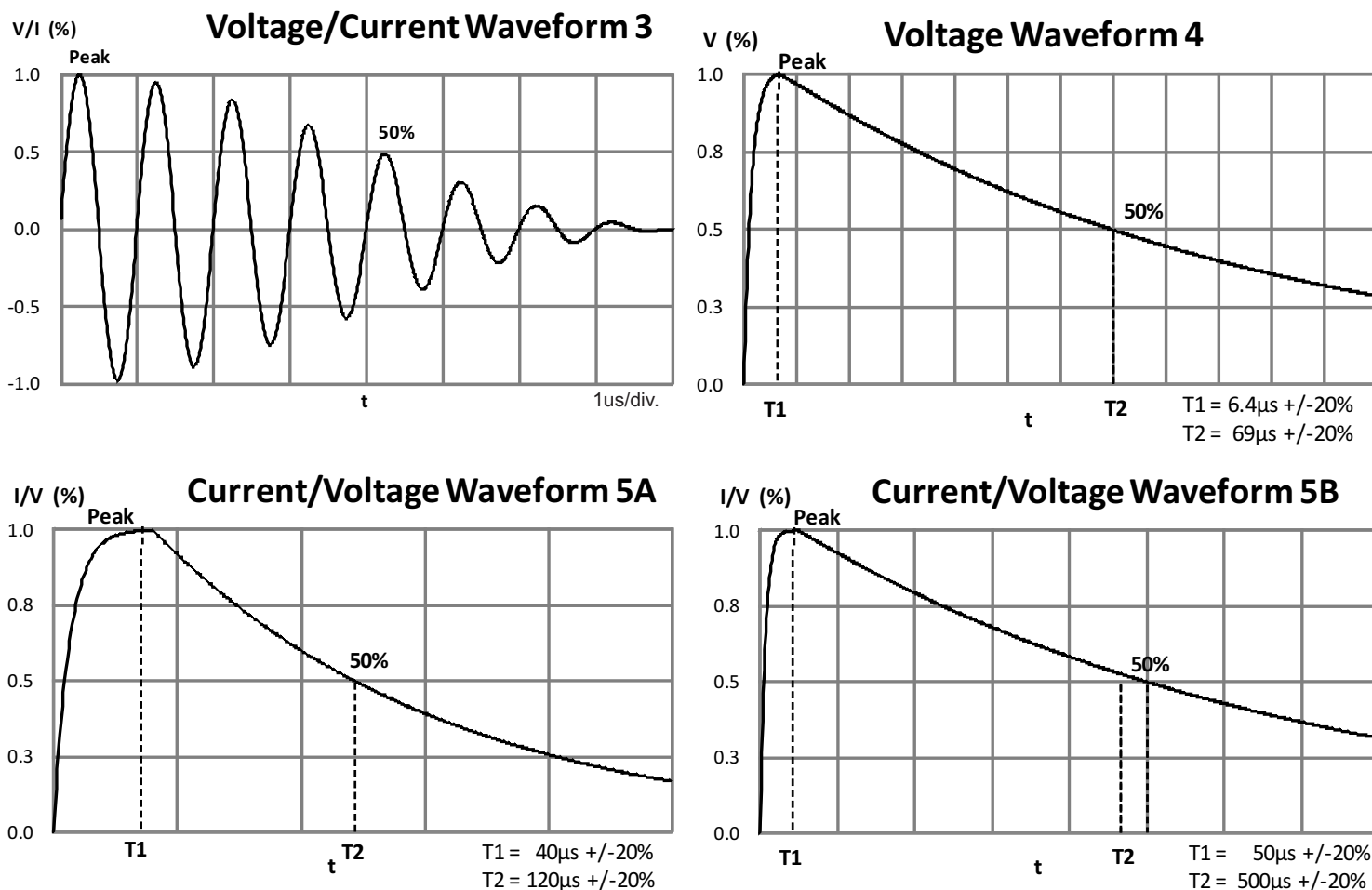
Figure 3. Lightning Waveforms
