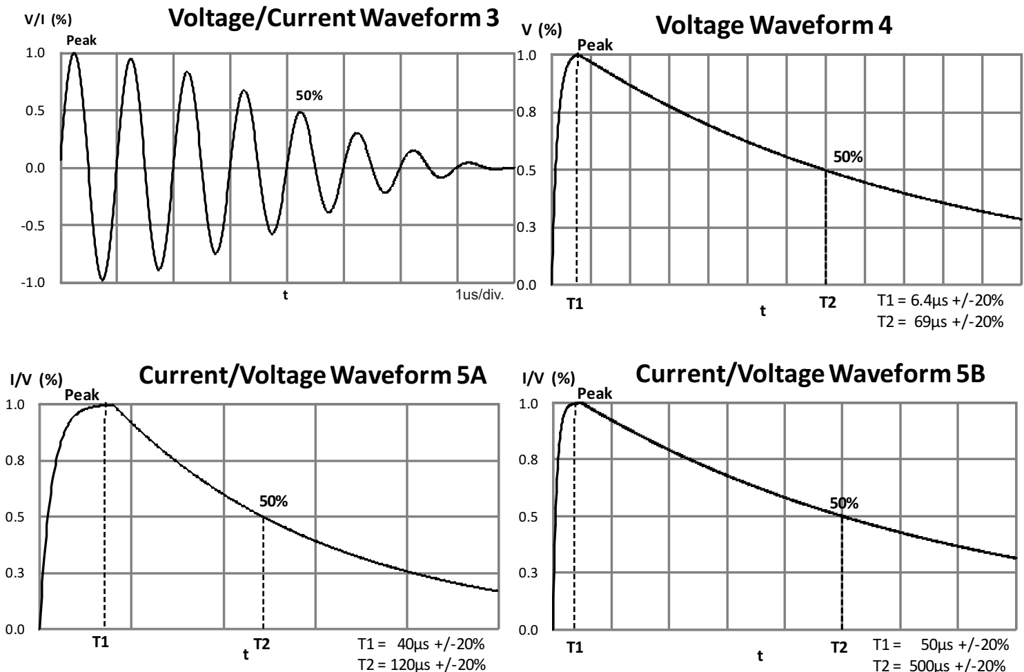
Figure 10. Lightning Waveforms
