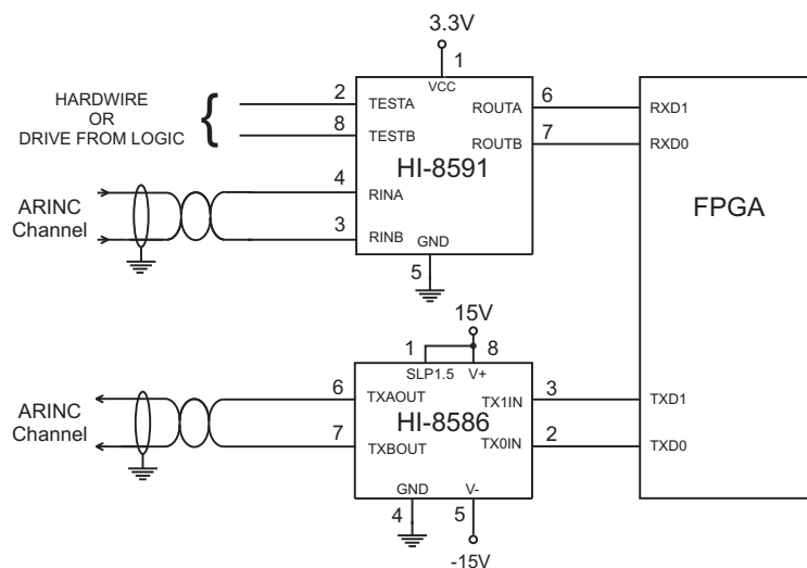
FIGURE 2 - APPLICATION DIAGRAM
