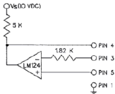
Figure 1 Heater Control Circuit
