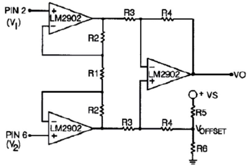
Figure 3 Differential Instrumentation Amplifier Circuit
