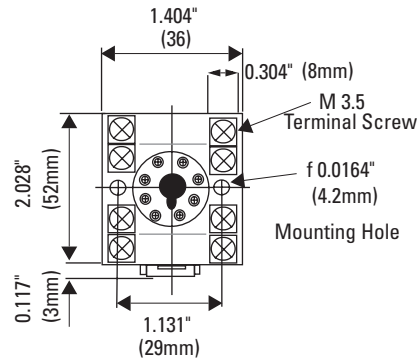
8-Pin SR2P-05
