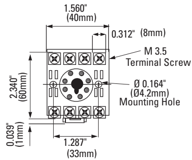
Terminal Arrangement
