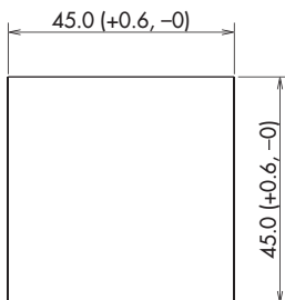
GE1A Timer Panel Cutout
