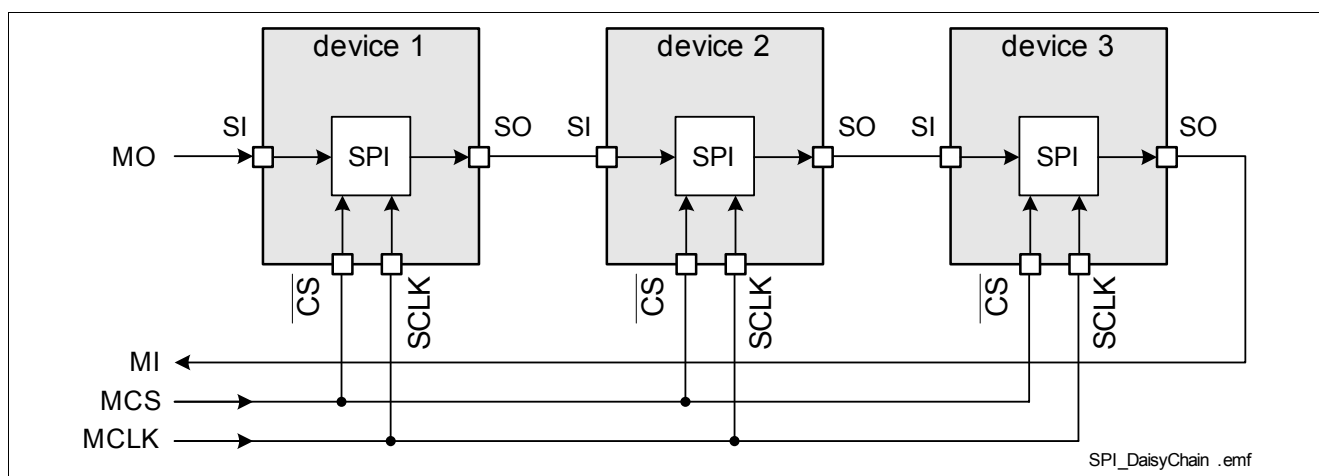
Figure 18 Daisy Chain Configuration
