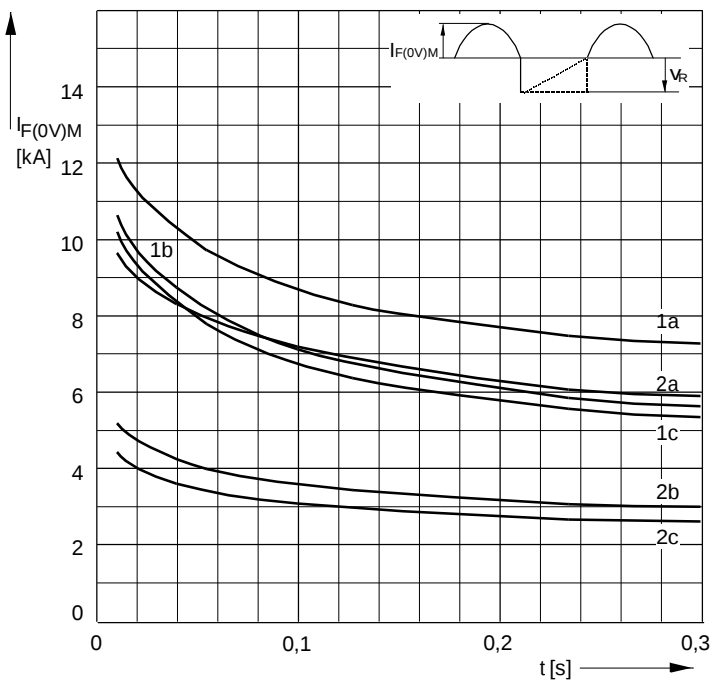
Bild / Fig. 4 Grenzstrom / Maximum overload forward current I_{F(0V)M} = f(t) 1 - I_{FAV(vor)} = 0\text{ A} ; t_{j} = t_{c} = 25\text{ °C} 2 - I_{FAV(vor)} = 400\text{ A} ; t_{c} = 130\text{ °C} ; t_{j} = 180\text{ °C} a - V_R \leq 50\text{ V} b - V_R = 0,5 V_{RRM} c - V_R = 0,8 V_{RRM}
