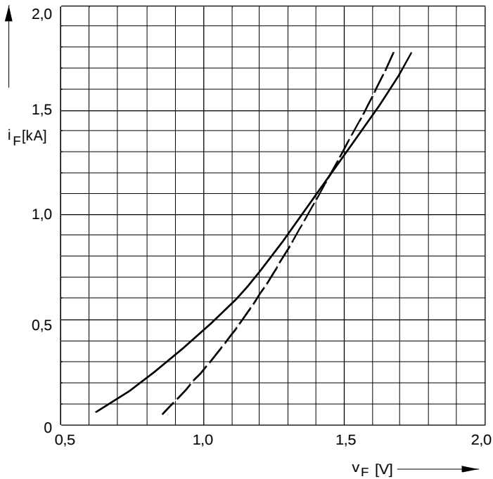
Bild/Fig. 1 Grenzdurchlaßkennlinie Limiting forward characteristic i_F = f(v_F) — t_{j} = 180\text{ °C} - - - t_{j} = 25\text{ °C}
