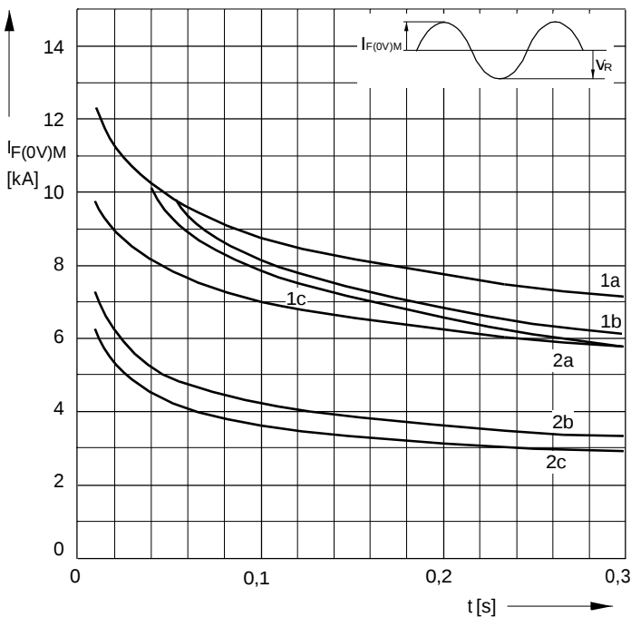
Bild / Fig. 3 Grenzstrom / Maximum overload forward current I_{F(0V)M} = f(t) 1 - I_{FAV(vor)} = 0\text{ A} ; t_{j} = t_{c} = 25\text{ °C} 2 - I_{FAV(vor)} = 400\text{ A} ; t_{c} = 130\text{ °C} ; t_{j} = 180\text{ °C} a - V_R \leq 50\text{ V} b - V_R = 0,5 V_{RRM} c - V_R = 0,8 V_{RRM}
