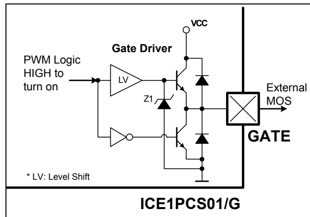
Figure 15 Gate Driver
