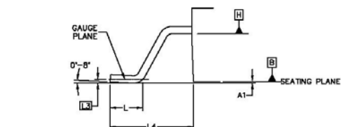
DETAIL "A" ROTATED 90° CW SCALE 8:1
