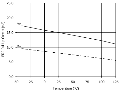
Figure 32A. ERR Pull-Up Current vs. Temperature
