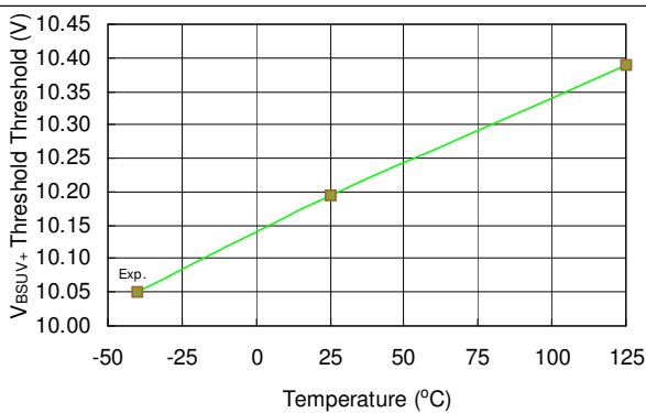
Figure 27. V BSVU+ Threshold vs. Temperature
