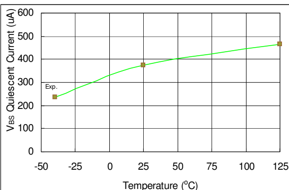
Figure 29. V BS Quiescent Current vs. Temperature
