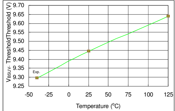
Figure 28. V BSVU- Threshold vs. Temperature
