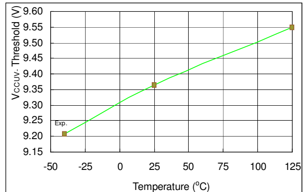
Figure 26. V CCUV- Threshold vs. Temperature
