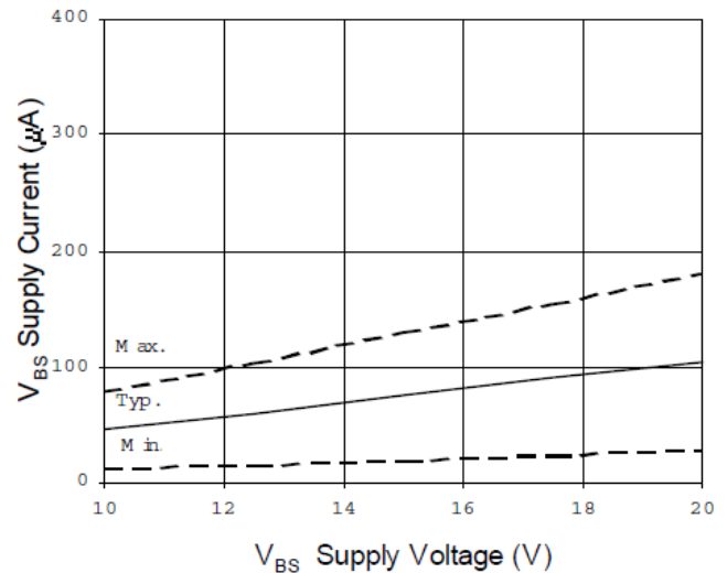
Figure 13B. V_{BS} Supply Current vs. Supply Voltage
