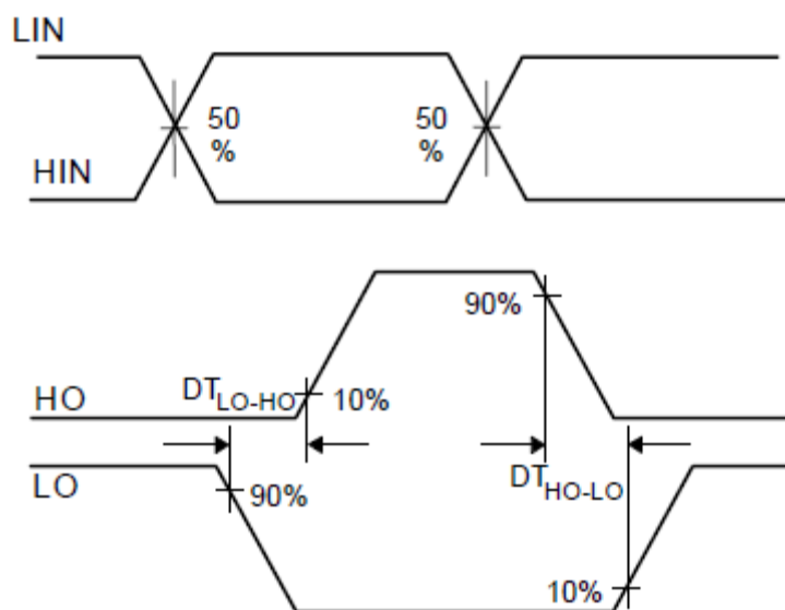
Figure 3. Deadtime Waveform Definitions
