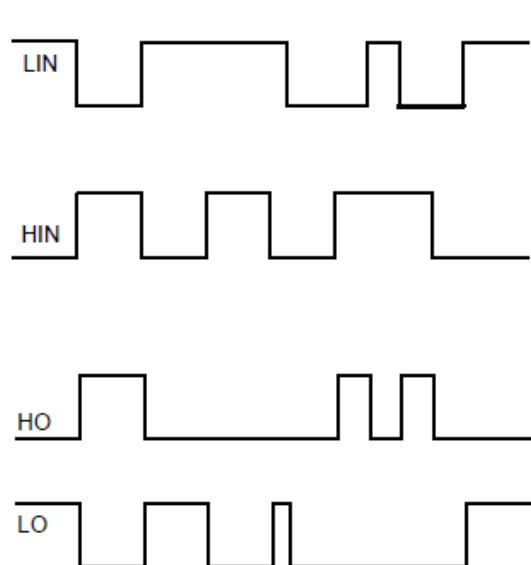
Figure 1. Input/Output Timing Diagram
