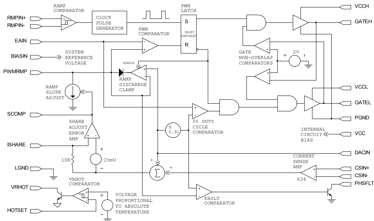
Figure 6. IR3088A Block Diagram
