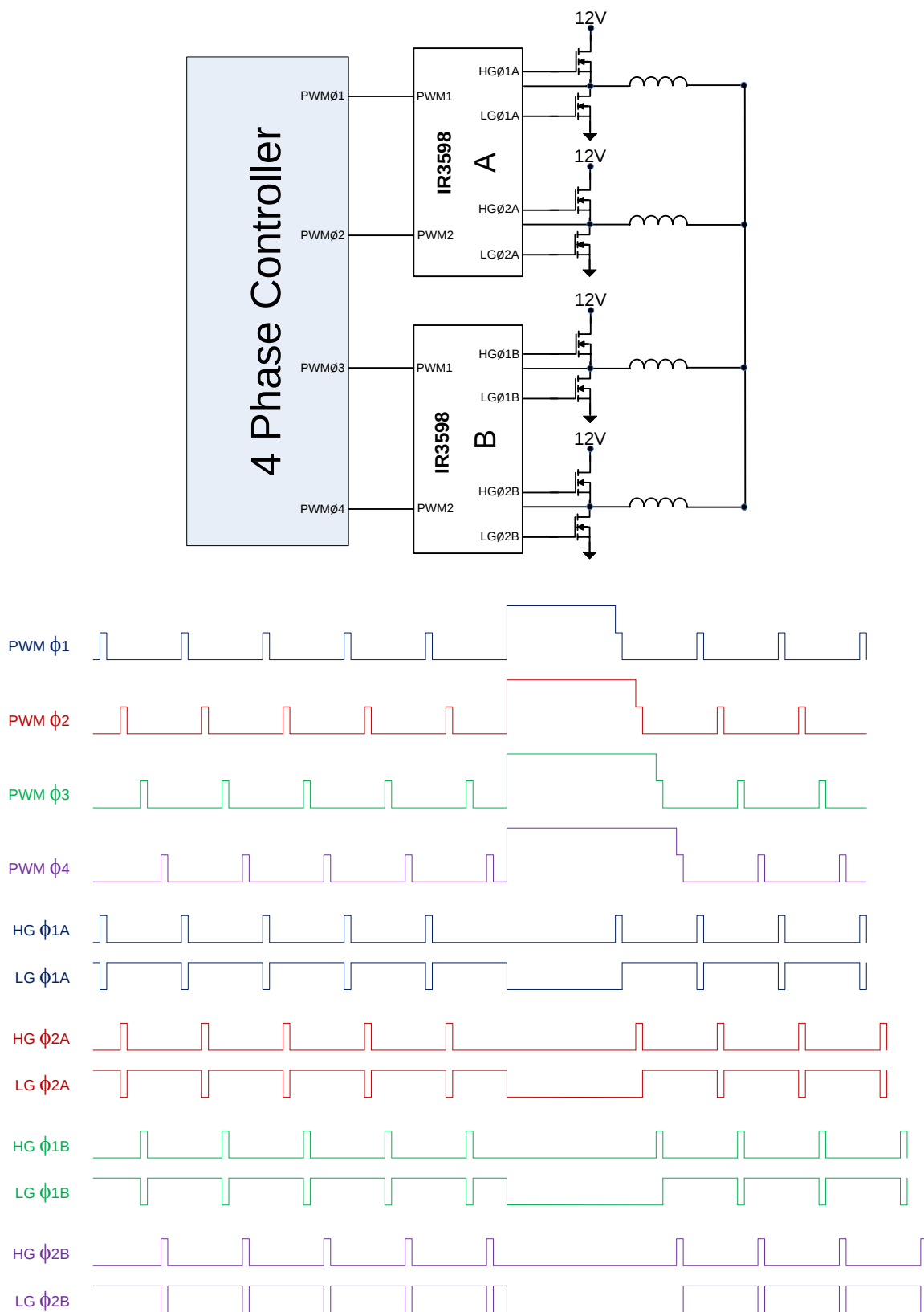
Figure 9: IR3598 timing when configured in DUAL mode (IR ATL PWM signals at input)
