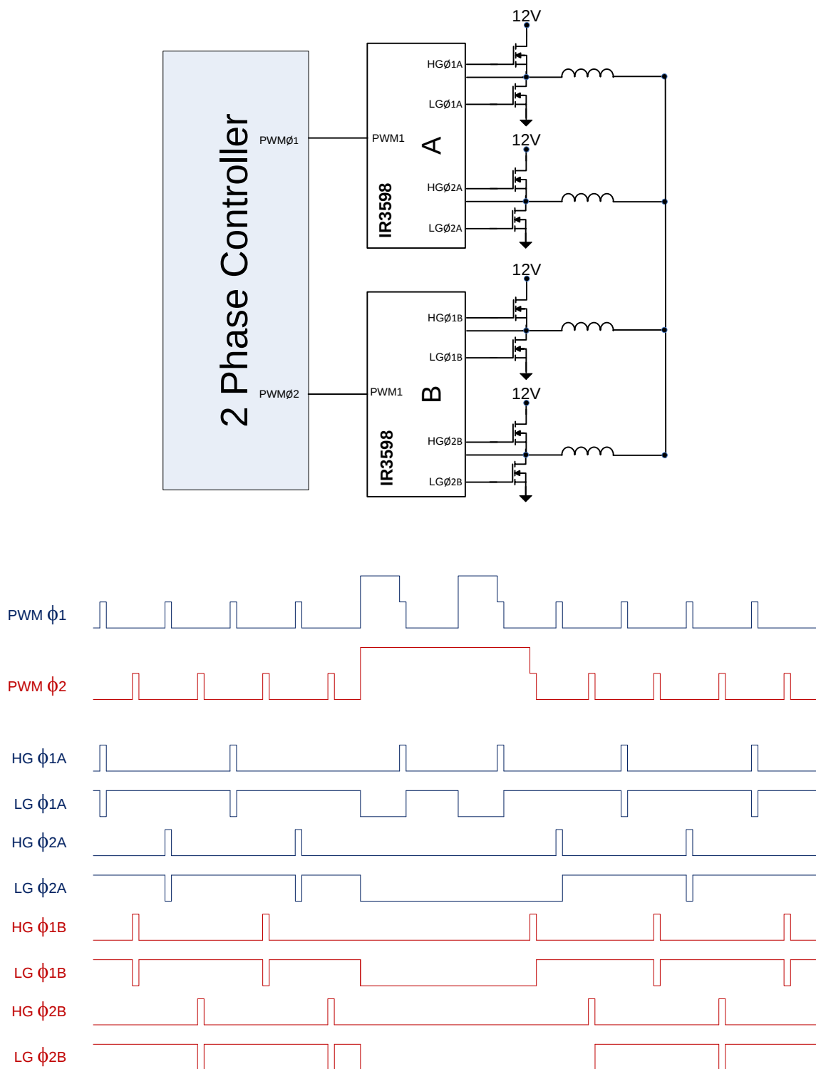
Figure 10: IR3598 timing when configured in DOUBLER mode (IR ATL PWM signals at input)
