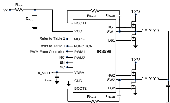
Figure 1: IR3598 Typical DOUBLER Mode Application Circuit
