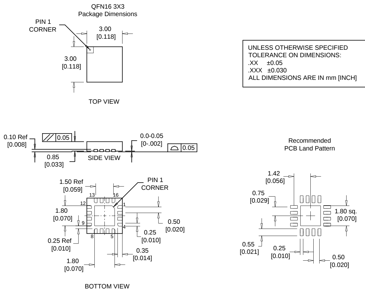
Figure 11: Package Dimensions
