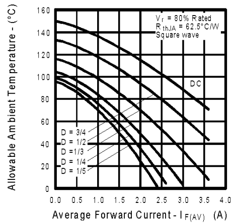
Fig. 14 - Maximum Allowable Ambient Temp. Vs. Forward Current
