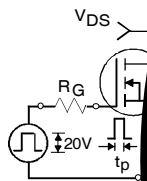
Fig 12a. Unclamped Inductive Switching (UIS)
