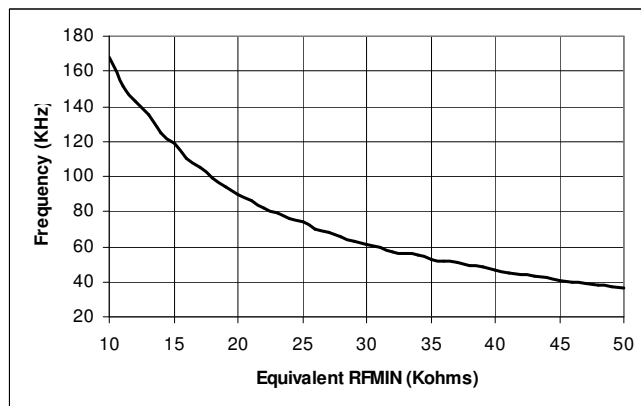
Figure 13: Graph of frequency against RFMIN
