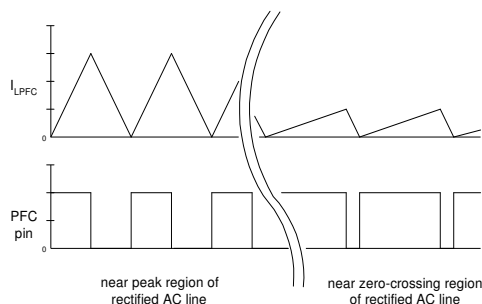
Figure 13: On-time modulation circuit timing diagram
