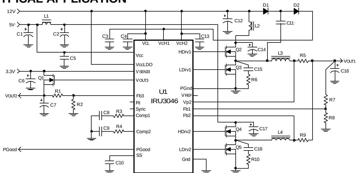
Figure 1 - Typical application of IRU3046 configured as 2-phase converter with current sharing.
