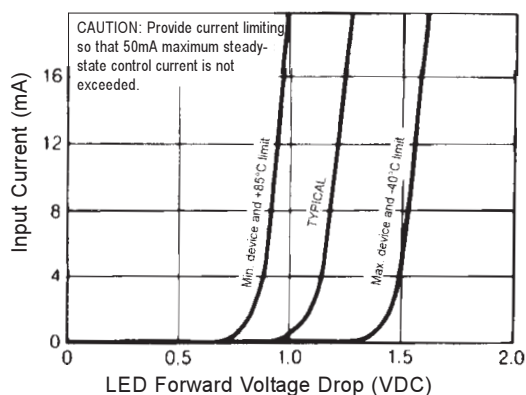
Figure 5. Input Characteristics
