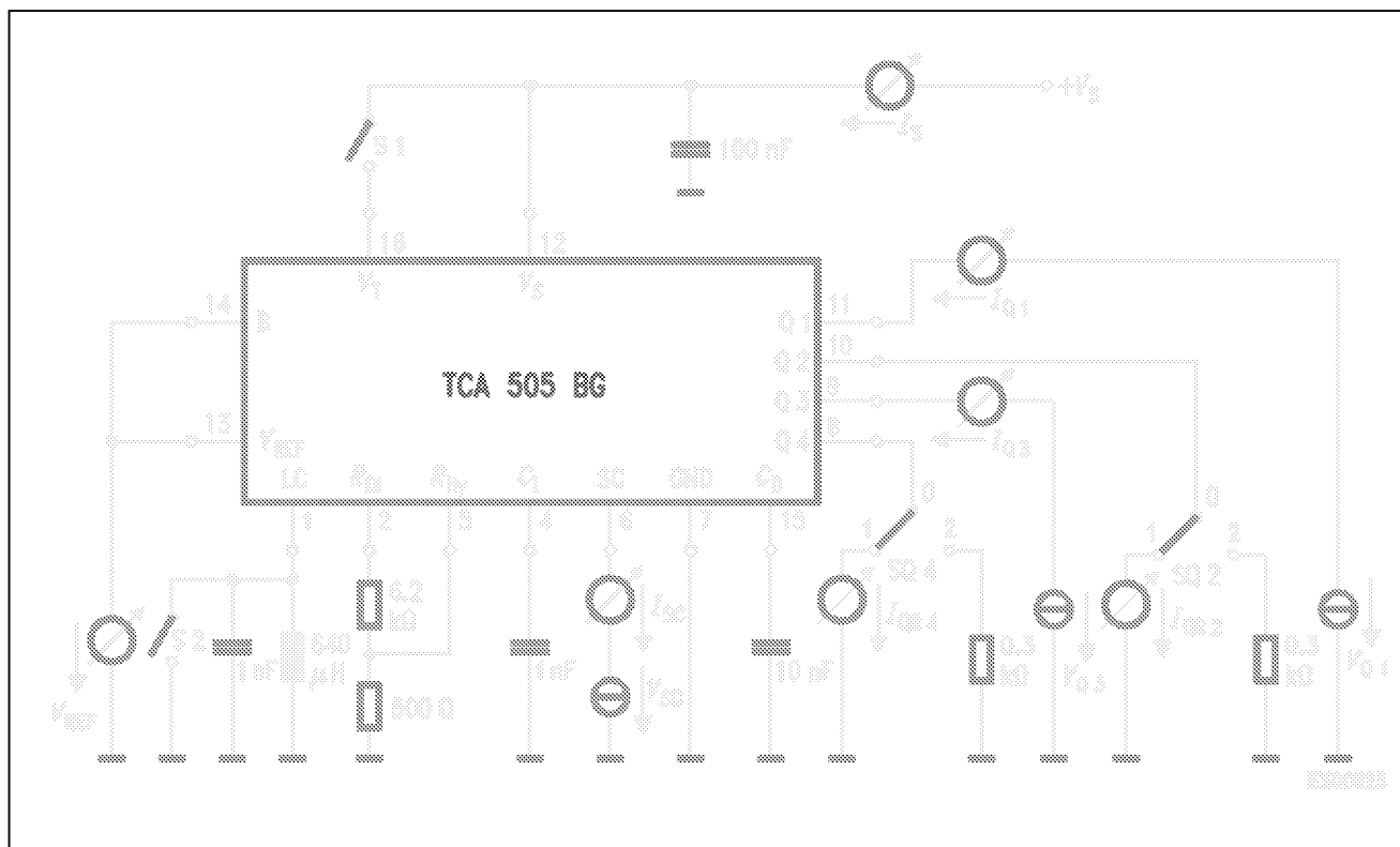
Test Circuit 1
