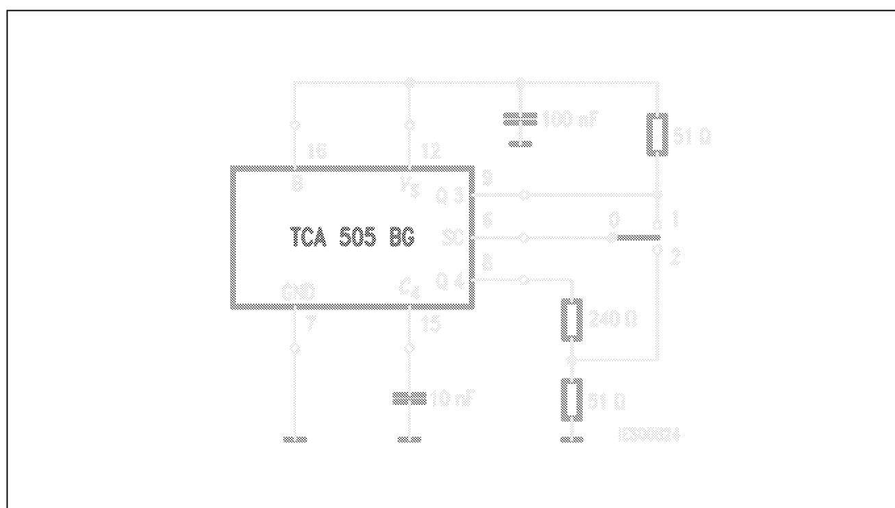
Test Circuit 2
