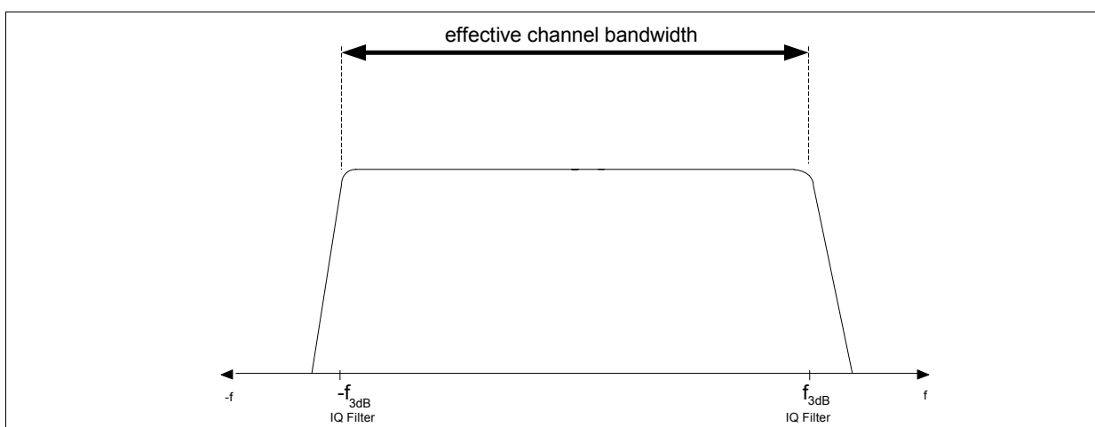
Figure 3-21 IQ Filter and frequency characteristics of the receive system
