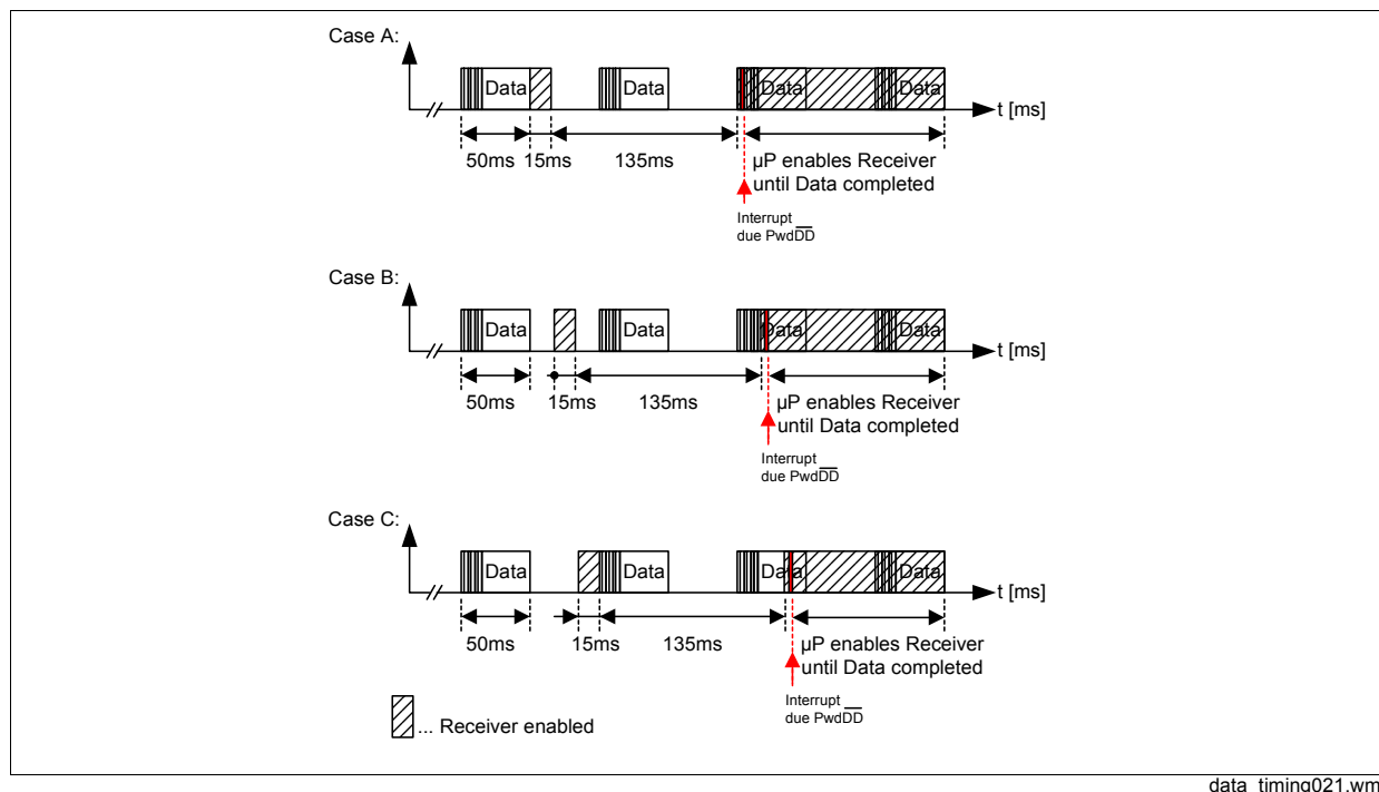
Figure 3-35 3 possible timings
