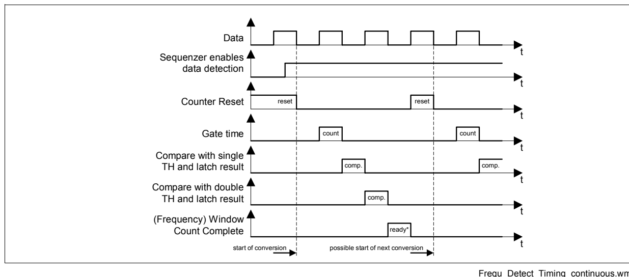
Figure 3-31 Frequency Detection timing in continuous mode
