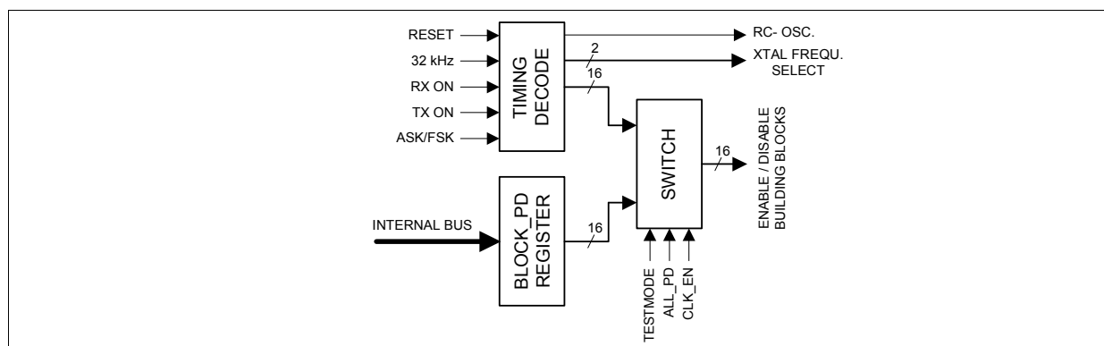
Figure 2-17 Sequencer's capability
