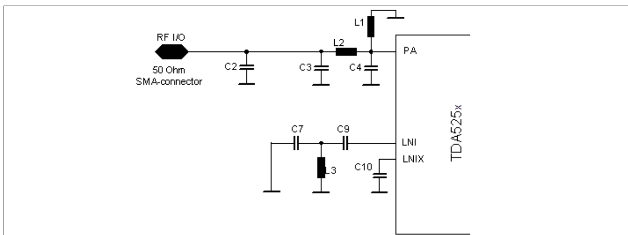
Figure 3-5 TX_Mode_simplified
