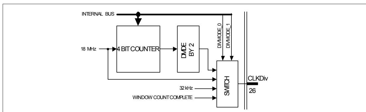
Figure 2-18 Clock Divider
