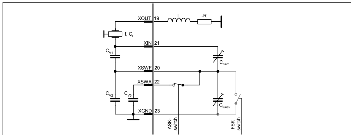
Figure 3-18 FSK receive
