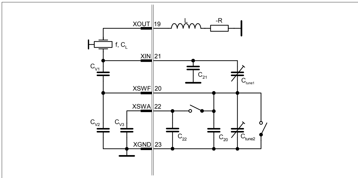
Figure 3-19 parasitics of the switching network
