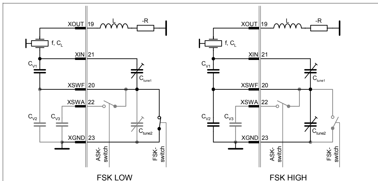
Figure 3-17 FSK modulation
