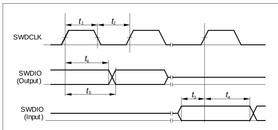
Figure 18 SWD Timing
