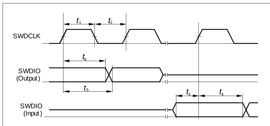
Figure 21 SWD Timing
