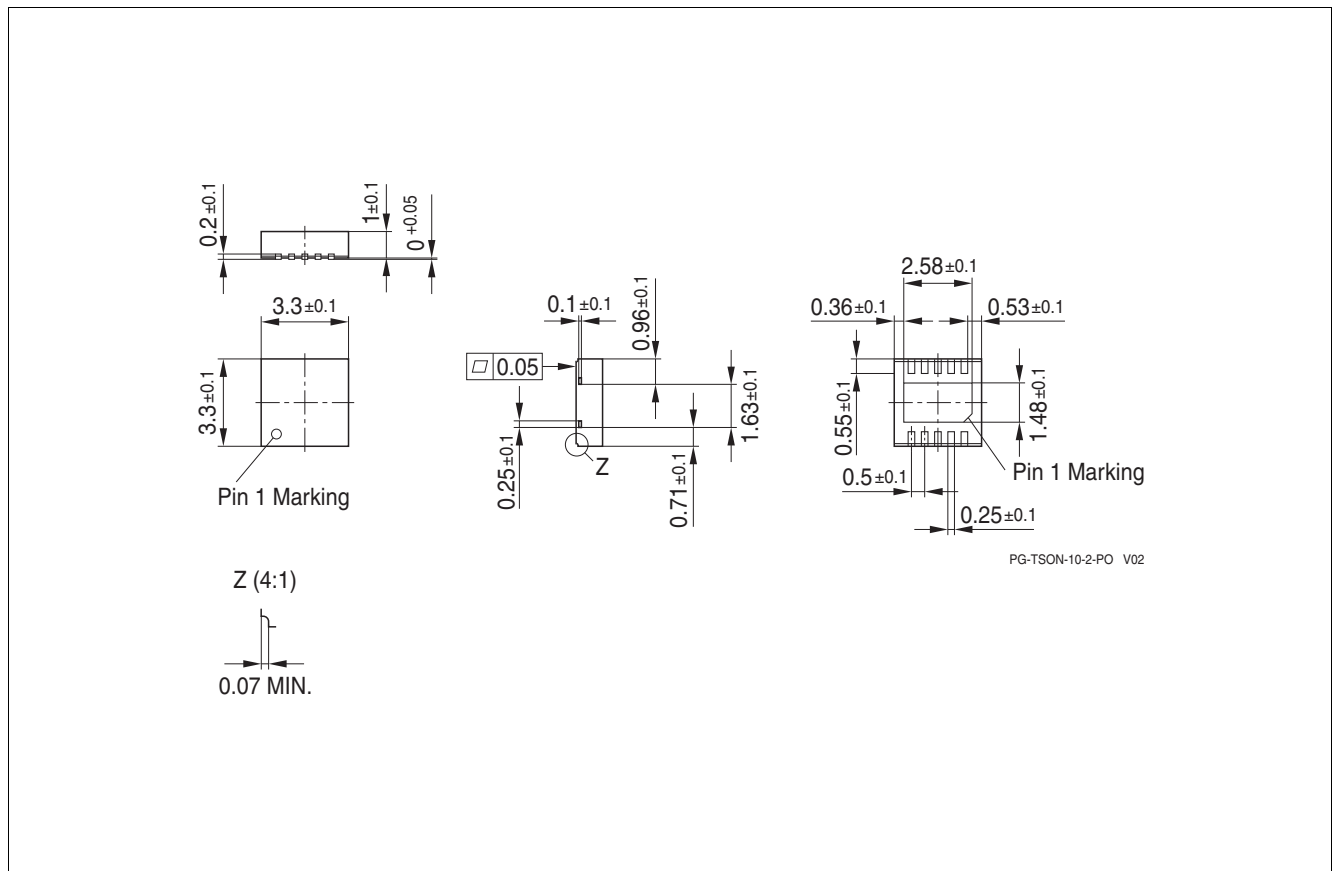
Figure 6 PG-TSON-10
