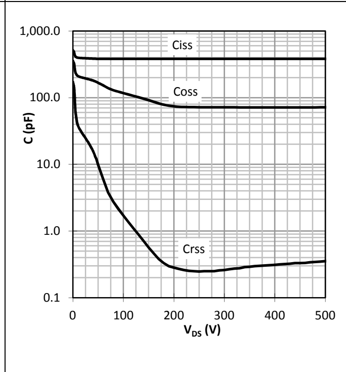
Figure 20 Typ. capacitances
