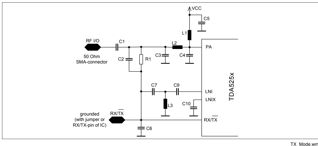
Figure 3-4 TX_Mode
