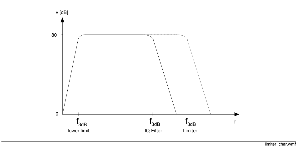
Figure 3-20 Limiter frequency characteristics
