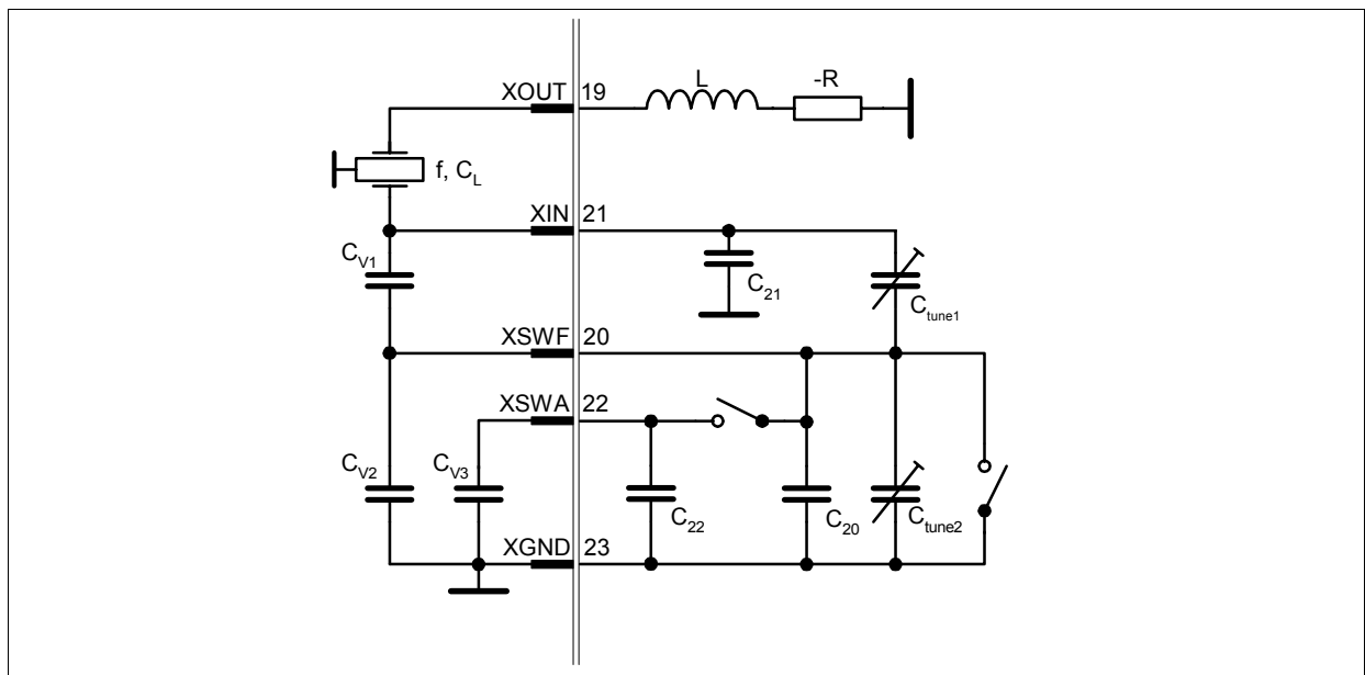
Figure 3-16 parasitics of the switching network
