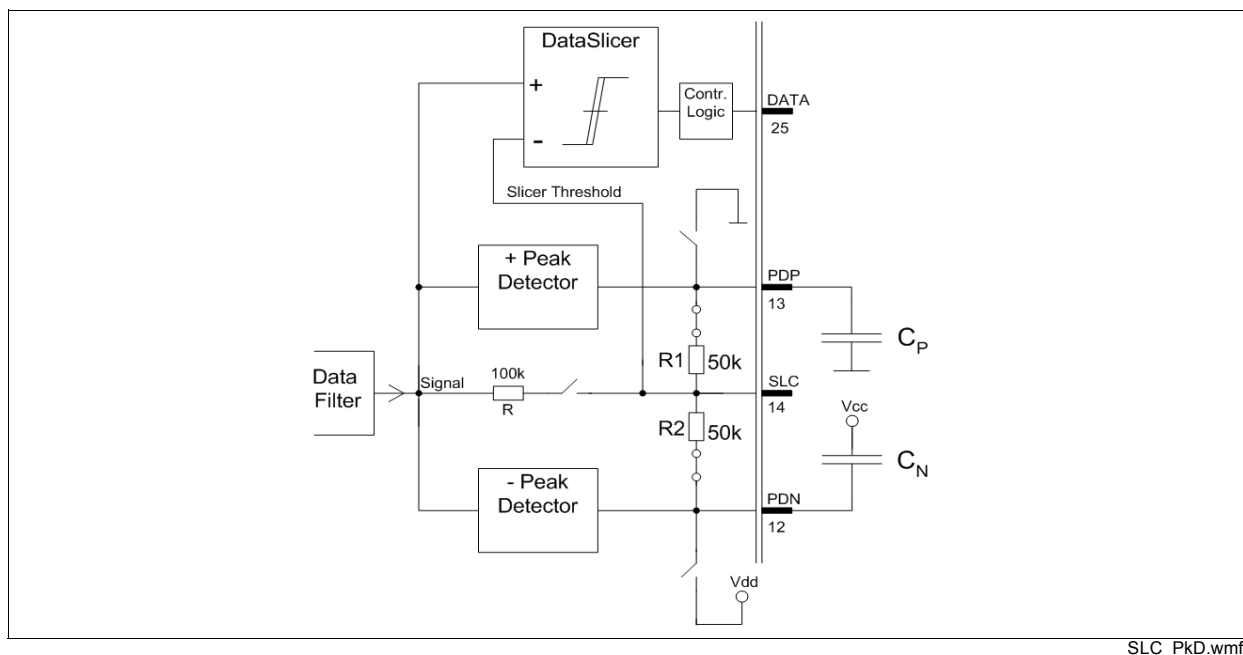
Figure 3-23 Slicer Level using Peak Detector
