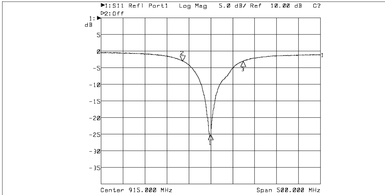
Figure 3-3 S11 measured
