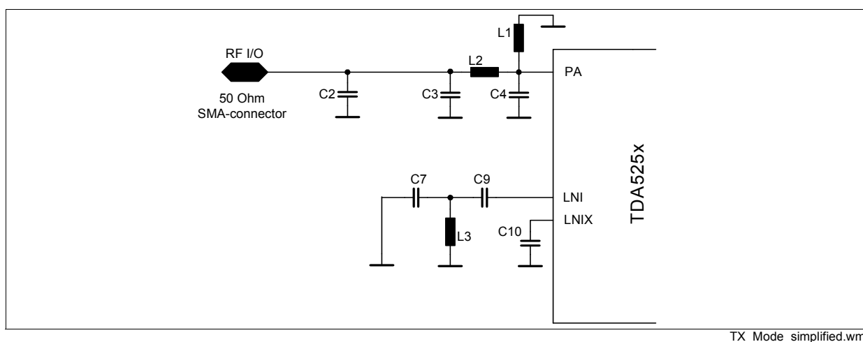
Figure 3-5 TX_Mode_simplified
