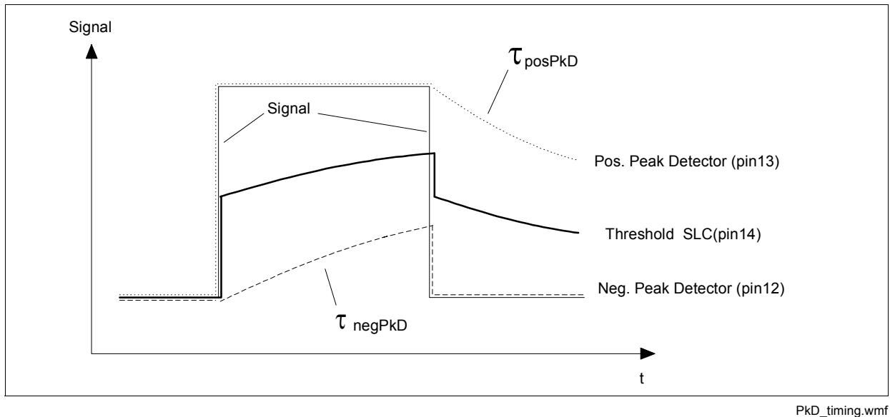
Figure 3-24 Peak Detector timing
