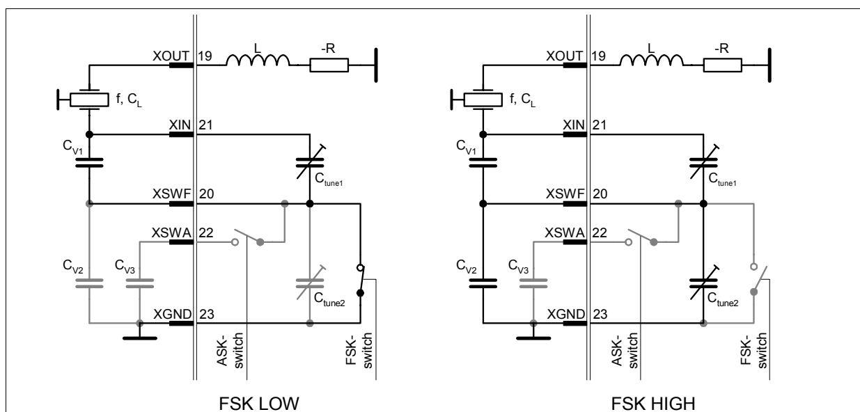
Figure 3-14 FSK modulation
