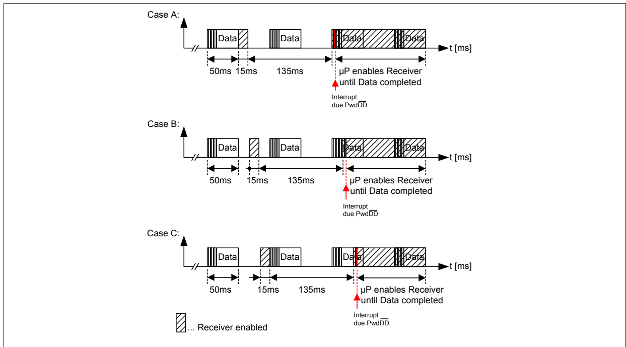
Figure 3-32 3 possible timings
