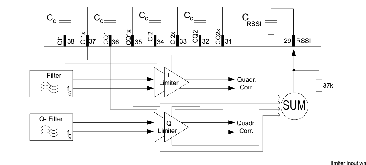
Figure 3-19 Limiter and Pinning
