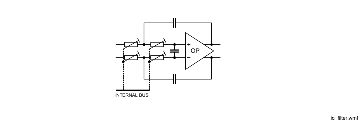
Figure 2-3 One I/Q Filter stage
