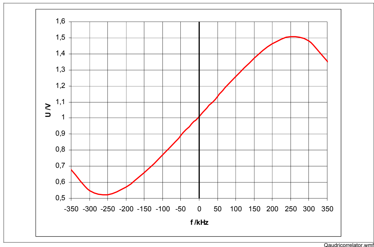
Figure 2-4 Typical Quadricorrelator Demodulation Characteristic
