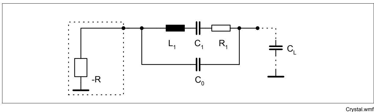
Figure 3-11 Crystal
