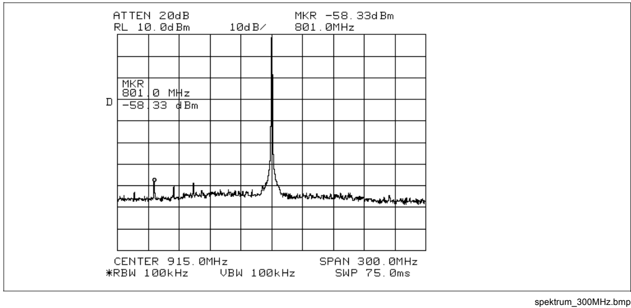
Figure 3-10 Transmit Spectrum 300MHz
