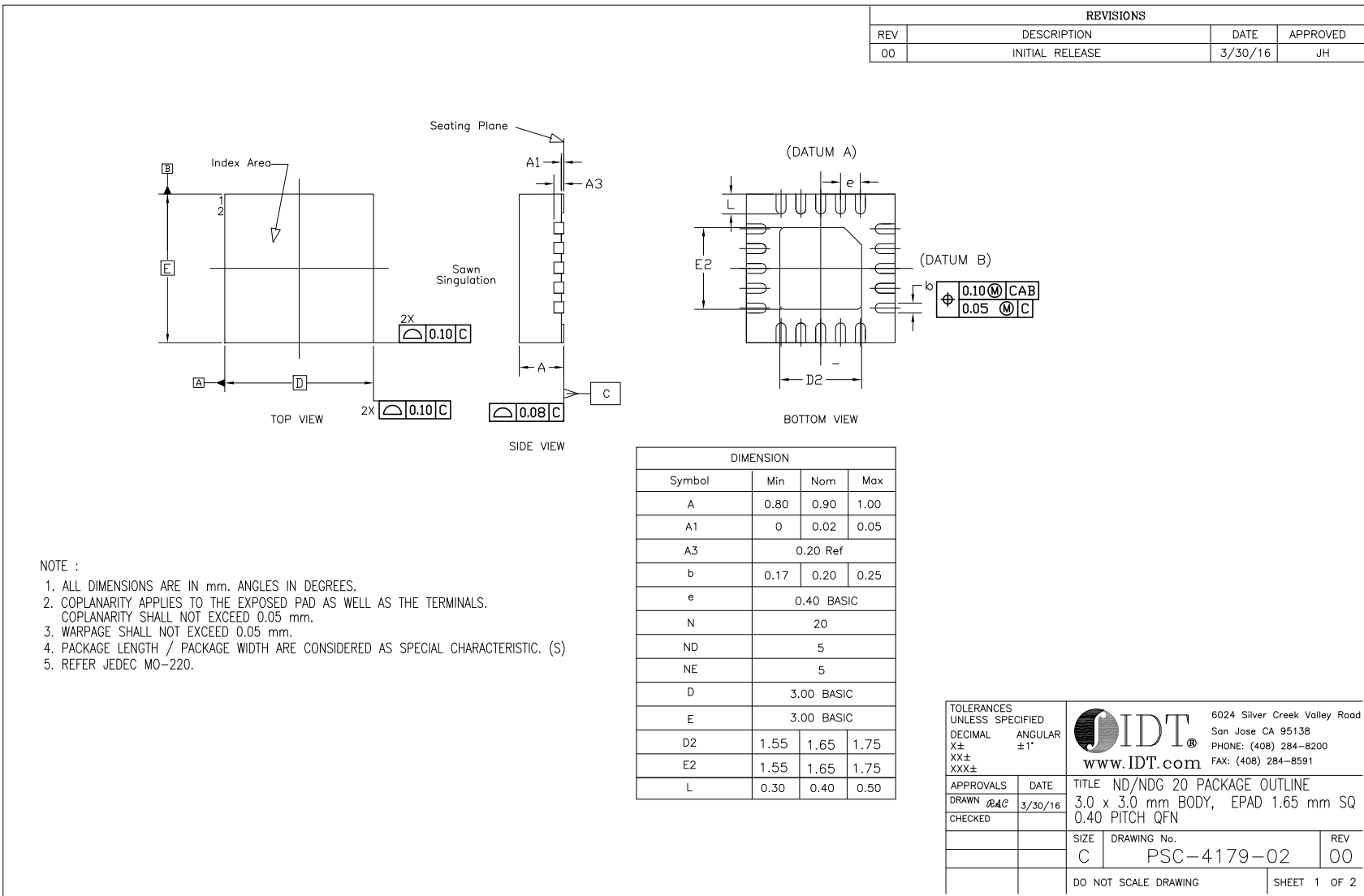
Figure 9. 3 x 3 mm 20-QFN Package Drawings–page 1
