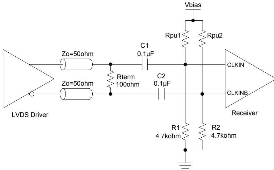
CLKIN, CLKINB Input Driven by an LVDS Driver
