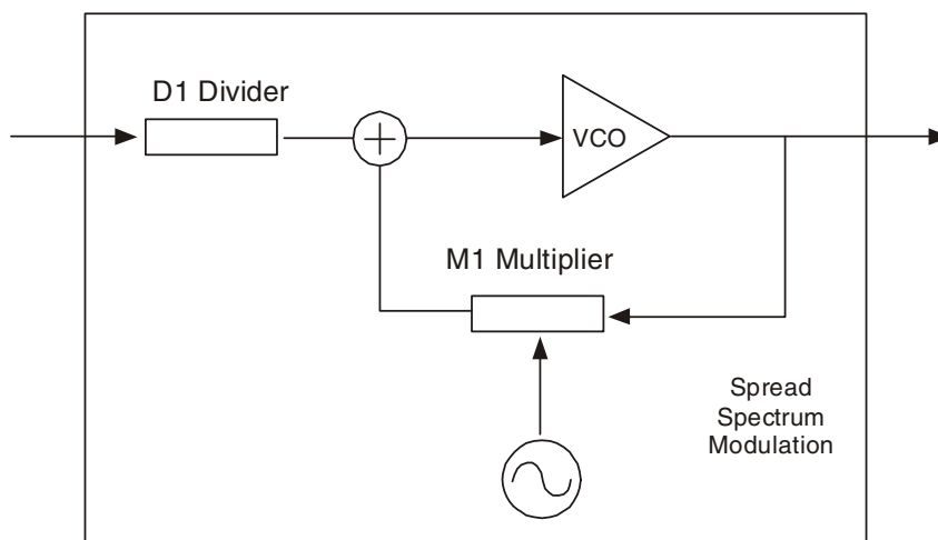
PLL1 Block Diagram
