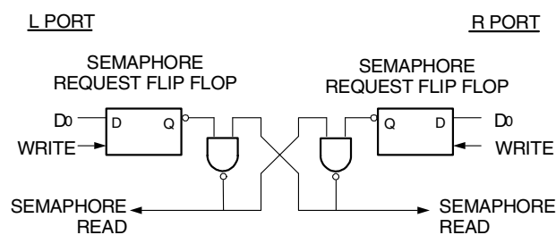
Figure 4. IDT7037 Semaphore Logic
