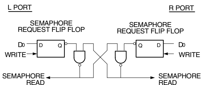
Figure 4. IDT70V18 Semaphore Logic
