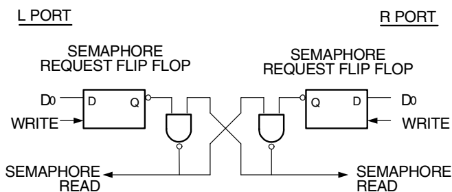
Figure 4. IDT70V37 Semaphore Logic
