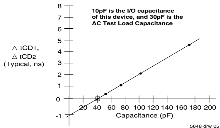
Figure 3. Typical Output Derating (Lumped Capacitive Load).
