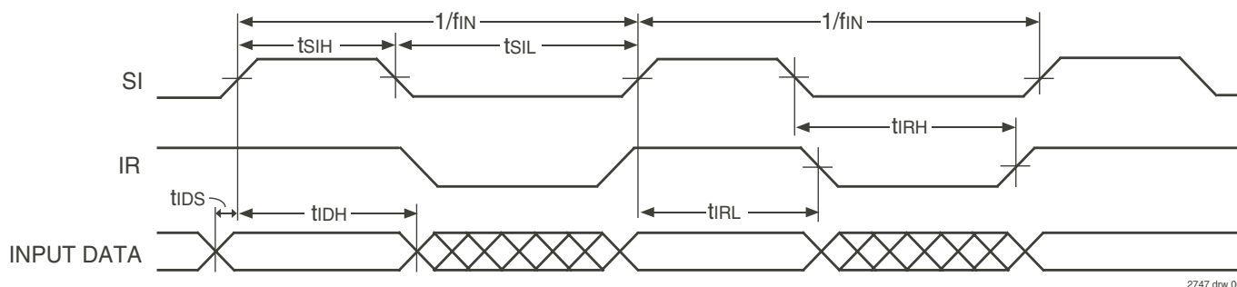
Figure 2. Input Timing
