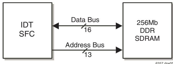
Figure 2b (1) . Configuration 2 - Two Chip Solution
