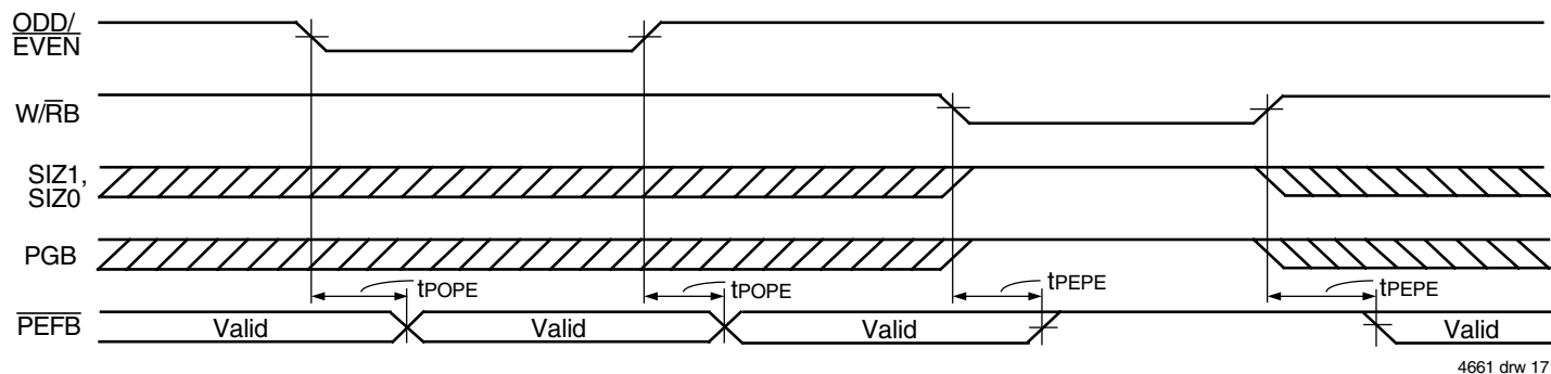
Figure 17. ODD/ EVEN , W/ RB , SIZE1, SIZE0, and PGB to PEFB Timing
