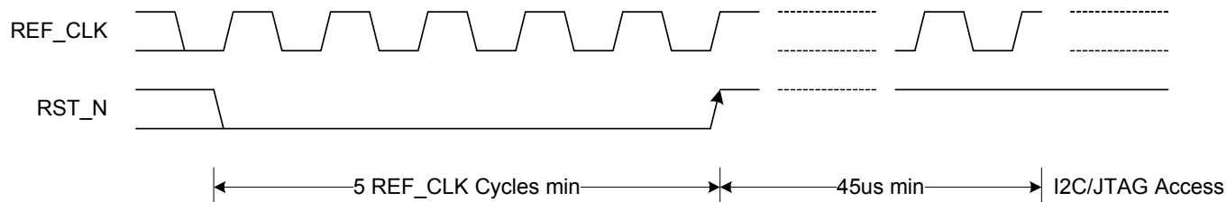
Figure 23: Reset Timing
