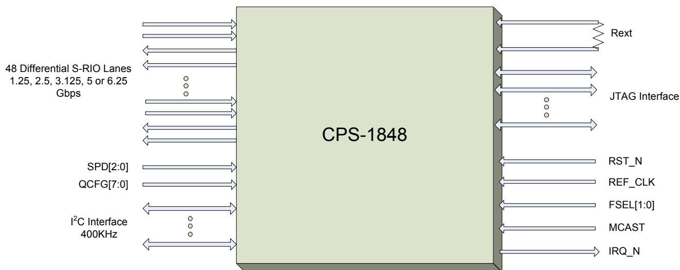
Figure 1: CPS-1848 Interfaces
