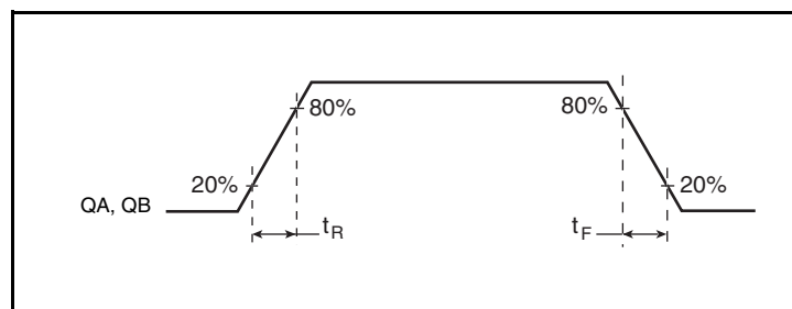
LVC MOS Output Rise/Fall Time
